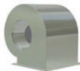
Fan 600w high power centrifugal fan. Running current 6.8A (max) 230v 50/60Hz 1pH
